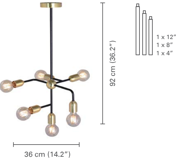
5-90211 SKYLIGHT Hauteur ajustable - comprend 3 tiges Adjustable height - includes 3 stems
